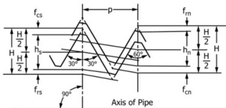
Taper 1 in 32 on Diameter (Shown Exaggerated in Diagram)
